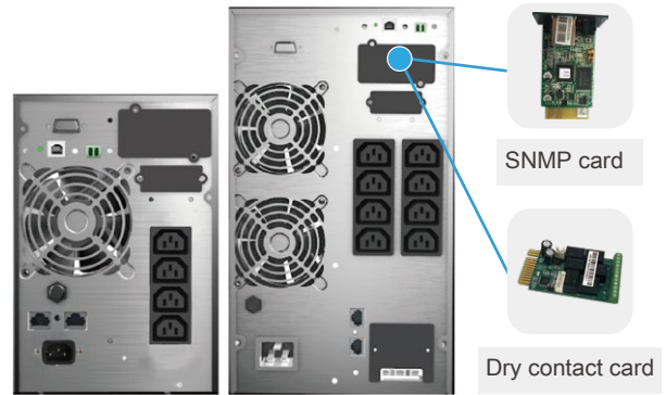
Rear Panel
